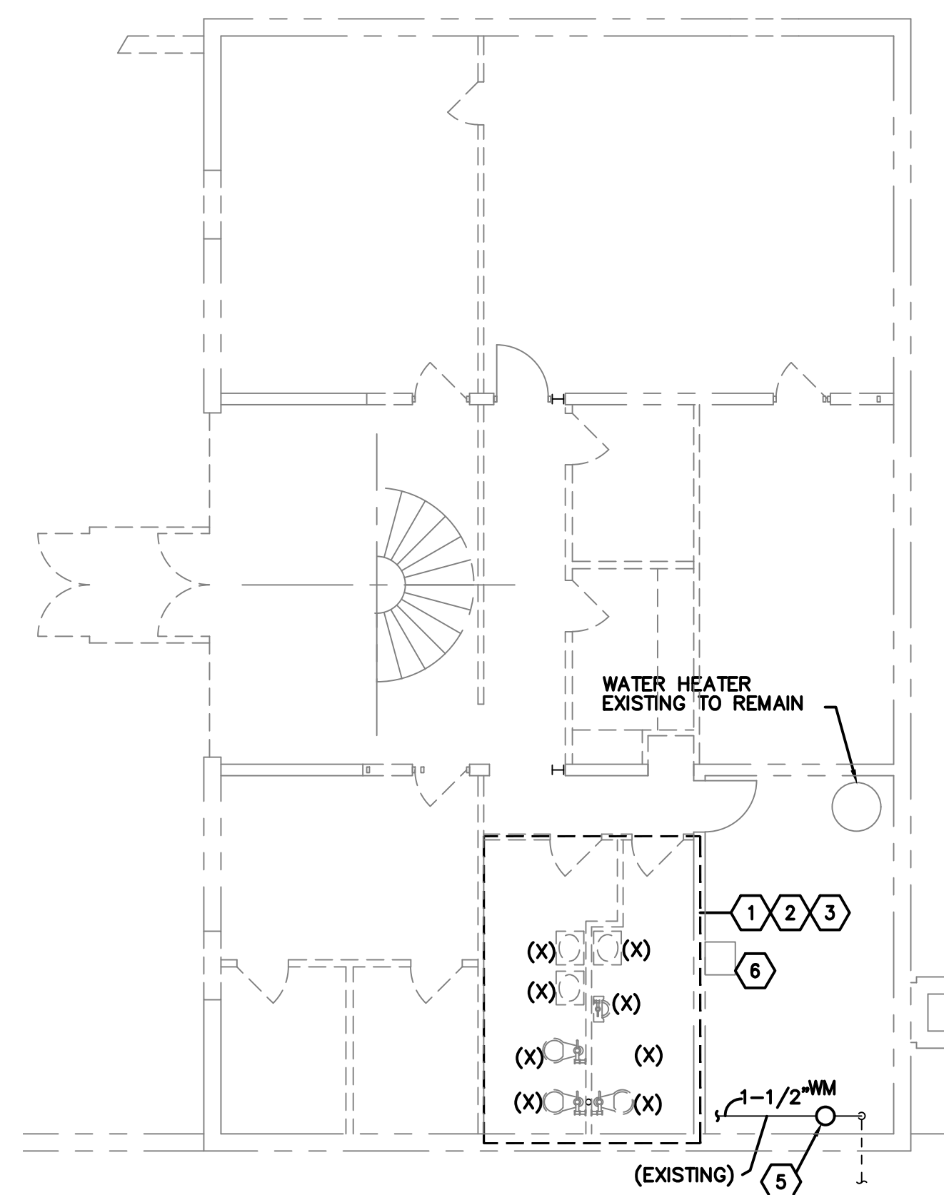
LOWER LEVEL PLUMBING DEMO FLOOR PLAN SCALE: 1/8" = 1'-0"
