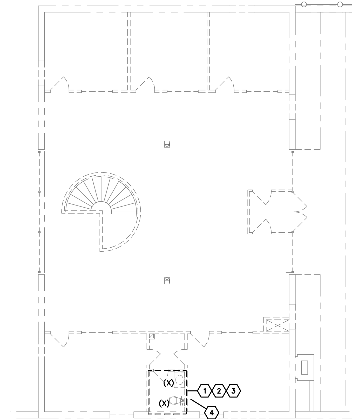
MAIN LEVEL PLUMBING DEMO FLOOR PLAN SCALE: 1/8" = 1'-0"
